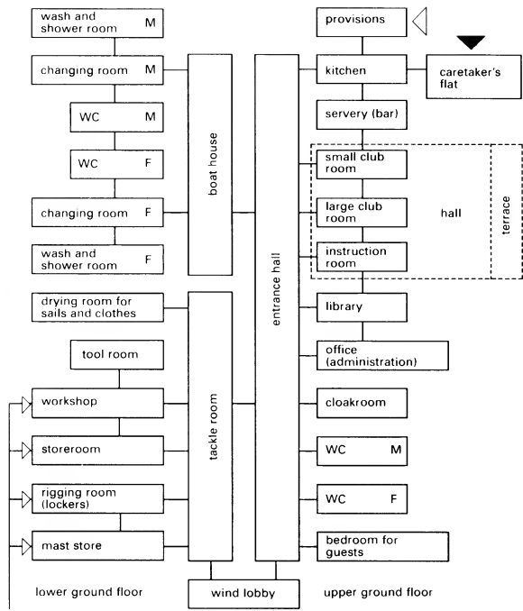
1 Functional diagram of a clubhouse
